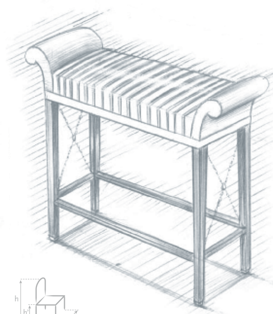
Tabouret "Diabolo" h 92 cm (3 ft), h' 87 cm (2.8 ft), l 80 cm (2.6 ft), p 50 cm (1.6 ft)
